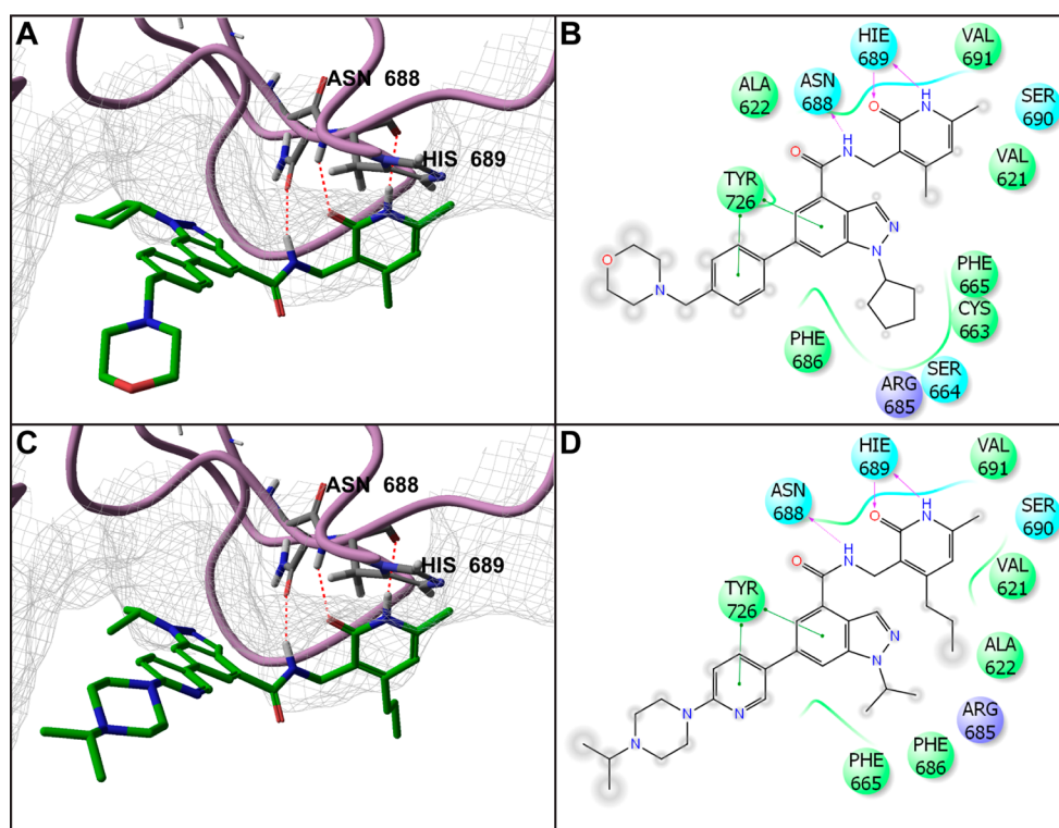
Figure 1. Binding hypothesis: UNC1999 binds to EZH2 similarly as EPZ005687, and its N -isopropyl piperazine moiety is solvent exposed. A homology model of EZH2 was constructed using GLP as a template (PDB: 2RF1). (A) EPZ005687 was docked into the SET domain; the ligand (green) orients such that the morpholine group is solvent exposed and therefore does not interact with EZH2 (purple). Additionally, there are three key hydrogen bonds that appear to be requisite for activity (dotted red lines). (B) Proposed ligand interactions of EPZ005687 display a hydrogen bond between the middle amide and Asn688 and two hydrogen bonds between the pyridone and His689 (purple arrows). (C) A docking model of UNC1999 shows it binds to EZH2 similarly as EPZ005687, and its N -isopropyl piperazine is solvent exposed. (D) Proposed ligand interactions of UNC1999 display the same key hydrogen bonds and hydrophobic interactions as EPZ005687.
