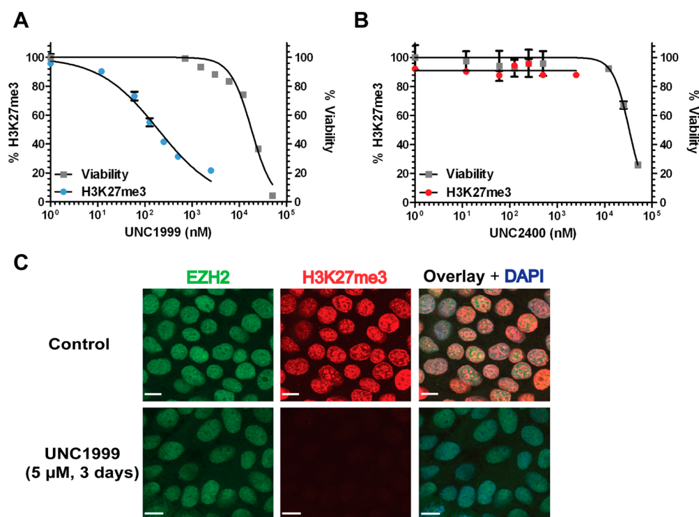
Figure 3. UNC1999 potently reduces H3K27me3 levels in cells and shows low cell toxicity. (A) UNC1999 reduces H3K27me3 levels in MCF10A cells with an IC_{50} = 124 \pm 11 nM ( n = 3 ) as determined by the ICW assay (blue) and displays low cell toxicity ( EC_{50} = 19,200 \pm 1200 nM ( n = 3 )) in the resazurin assay (gray). (B) UNC2400 displays negligible inhibition of H3K27me3 levels (red) in MCF10A cells while displaying toxicity ( EC_{50} = 27,500 \pm 1,300 nM ( n = 3 )) in the resazurin assay (gray) similar to that of UNC1999. (C) Immunofluorescence staining showed that treatment with UNC1999 (5 \mu M, 72 h) effectively reduced the H3K27me3 mark but did not affect EZH2 levels in MCF7 cells. Scale bar represents 10 \mu m.
