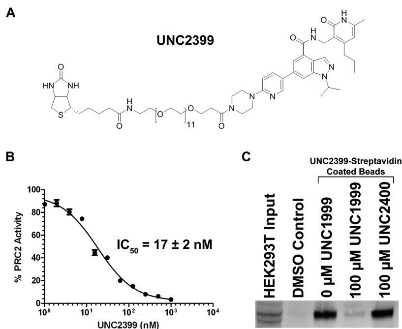
Figure 6. Biotinylated UNC1999 (UNC2399) enriches EZH2 from HEK293T cell lysates. (A) Structure of UNC2399, a biotinylated UNC1999. (B) UNC2399 displays high in vitro potency (IC 50 = 17 ± 2 nM) for EZH2. (C) In UNC2399 pull-down experiments EZH2 levels are markedly enriched (well 3) as compared to the DMSO control (well 2). The ability to pull-down EZH2 out of cell lysates is abolished by pretreatment with 100 μM UNC1999 (well 4) but is not affected by pretreatment with 100 μM UNC2400 (well 5). This western blot is representative of three biological replicates.
