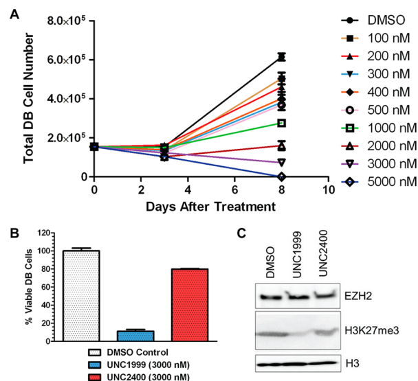
Figure 4. UNC1999 selectively kills DB cells, a DLBCL cell line with the EZH2 Y641N mutation. (A) UNC1999 displays a concentration- and time-dependent inhibition of DB cell proliferation ( EC_{50} = 633 \pm 101 nM ( n = 3 )). (B) UNC2400 (3000 nM, 8 days) does not significantly inhibit DB cell proliferation in contrast to UNC1999. (C) Western blotting of EZH2, H3K27me3, and H3 following the treatment of DB cells with UNC1999 or UNC2400 at 3000 nM for 3 days. UNC1999 decreases H3K27me3 but not EZH2 levels, while UNC2400 does not significantly reduce H3K27me3 or EZH2 levels in DB cells.
